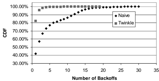
Figure 2: CDF of the number of backoffs due to contention with a normal “naive” application, and the same traffic using Twinkle. (Both use the same CSMA Mac.)
