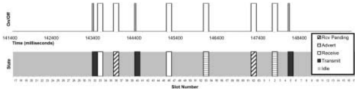
Figure 6: A subsection of the validation experiment. The bottom graph shows the measured Twinkle state versus time and the slot number; this section shows about one cycle with 64 slots per cycle and 128ms slots. The top graph shows actual radio on/off times. Note that the radio is always off for Idle cycles and that for Transmit cycles the on time is just long enough to transmit the queued messages.
